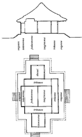
3.39 Distinct spatial layers in the central hall of the Ho-o-den.
